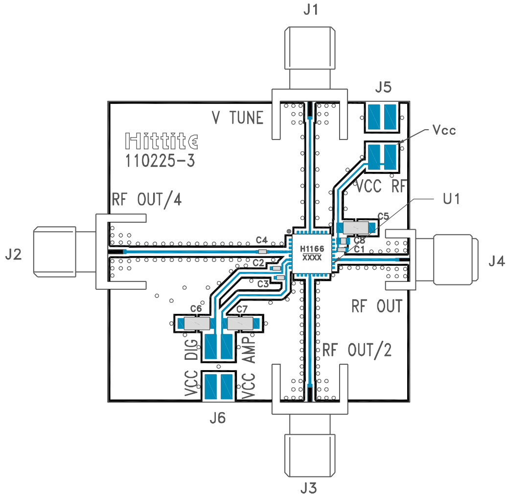
Figure 17. Evaluation PCB
